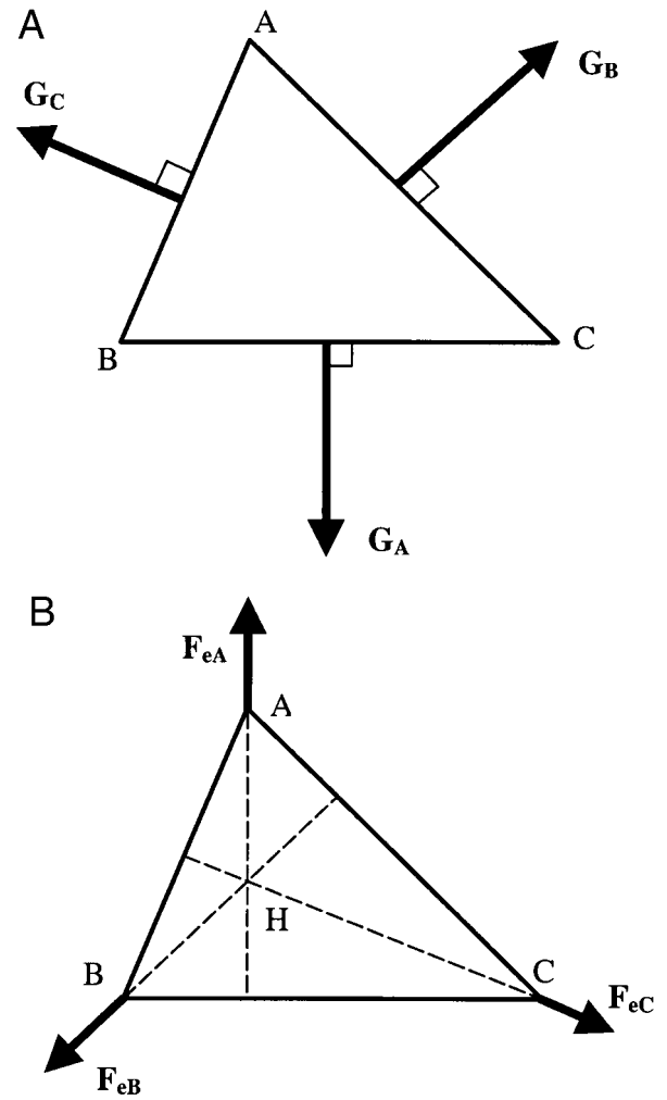
FIGURE 11 (A) Configuration of three forces \mathbf{G}_A , \mathbf{G}_B , and \mathbf{G}_C generating a pure expansion stress on the triangle ABC. They are oriented along the normals to the segments BC, CA, and AB, and their sum \mathbf{G}_A + \mathbf{G}_B + \mathbf{G}_C is zero. (B) The three forces \mathbf{F}_{eA} , \mathbf{F}_{eB} , and \mathbf{F}_{eC} applied at the vertices A, B, and C exert a pure expansion stress equivalent to the one generated by \mathbf{G}_A , \mathbf{G}_B , and \mathbf{G}_C . They are supported by the triangle heights and their amplitude is given by equations A5–A7.
